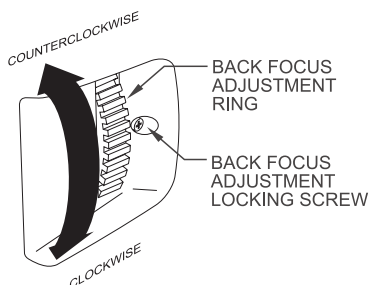
Figure 7. Back Focus Adjustment
